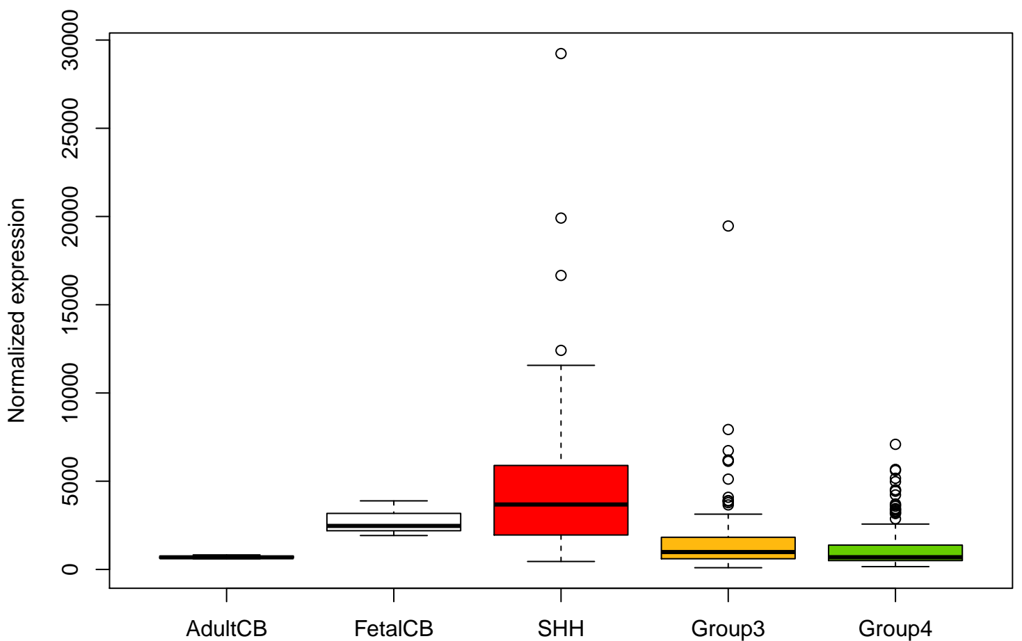
CTSC ENSG00000109861 expression (including outliers)
