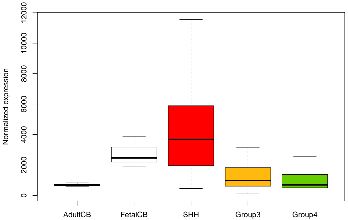
CTSC ENSG00000109861 expression (no outliers)
