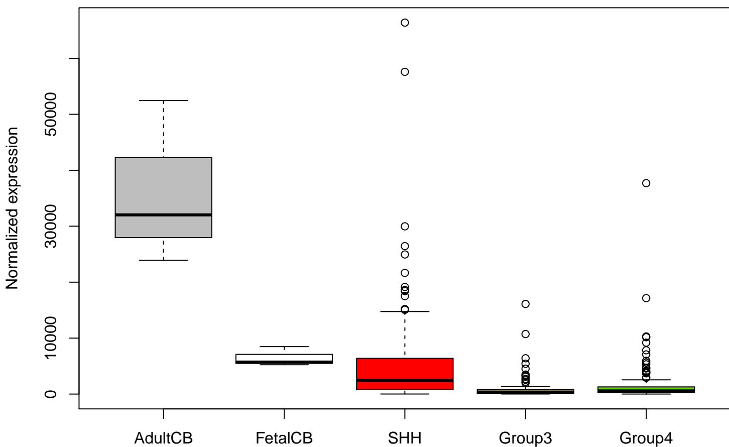
CALN1 ENSG00000183166 expression (including outliers)
