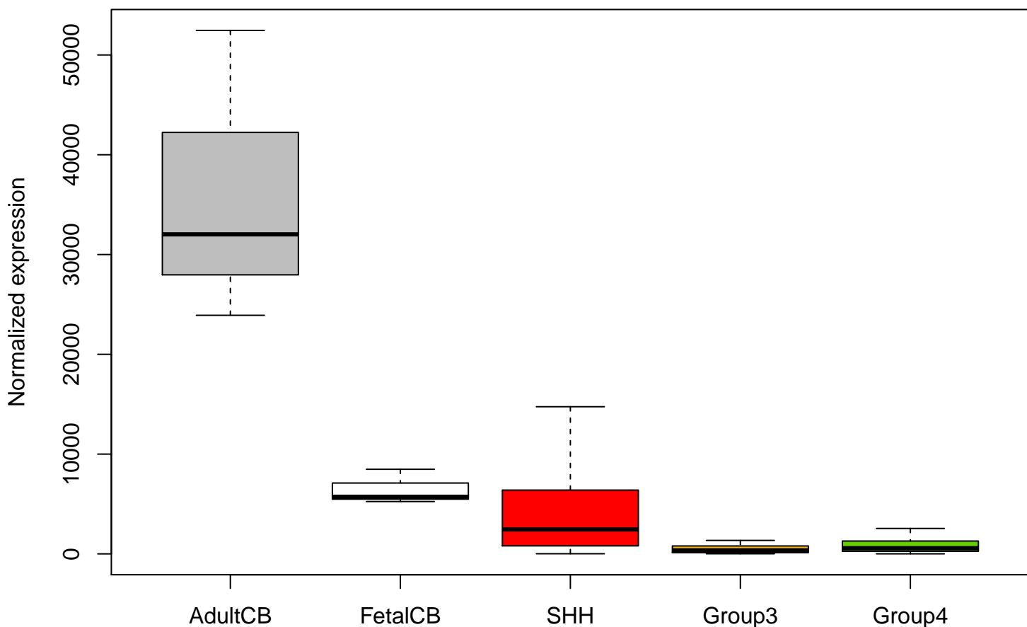
CALN1 ENSG00000183166 expression (no outliers)
