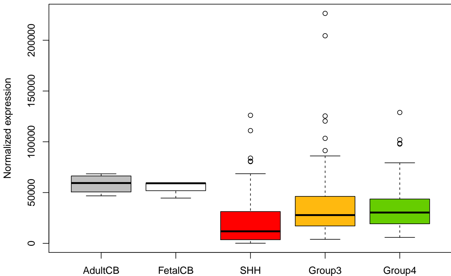
L1CAM ENSG00000198910 expression (including outliers)
