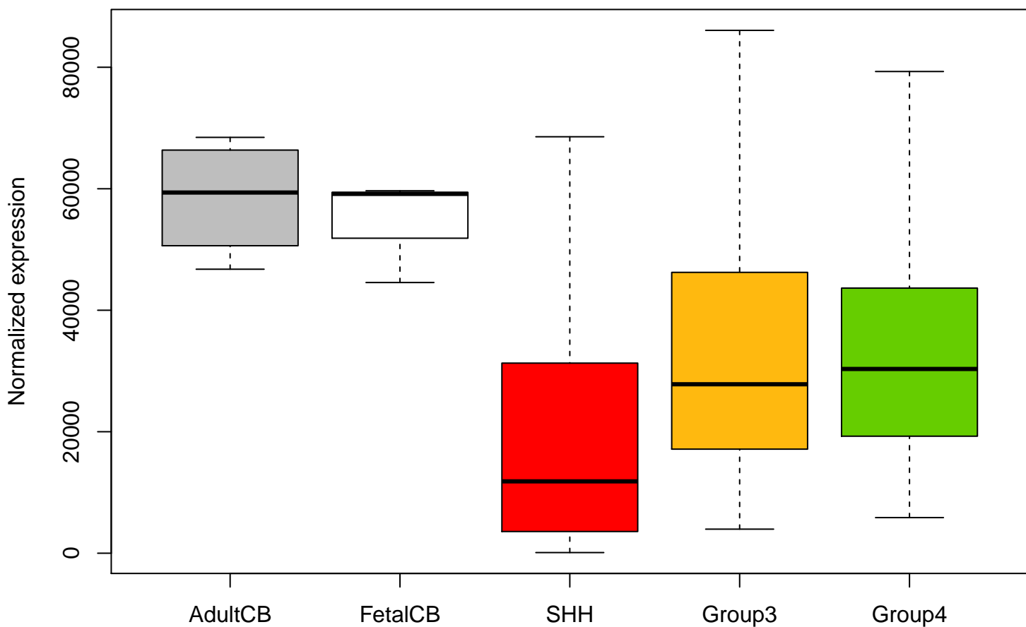
L1CAM ENSG00000198910 expression (no outliers)
