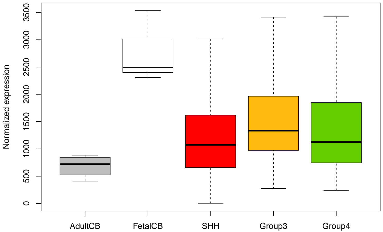
KDR ENSG00000128052 expression (no outliers)
