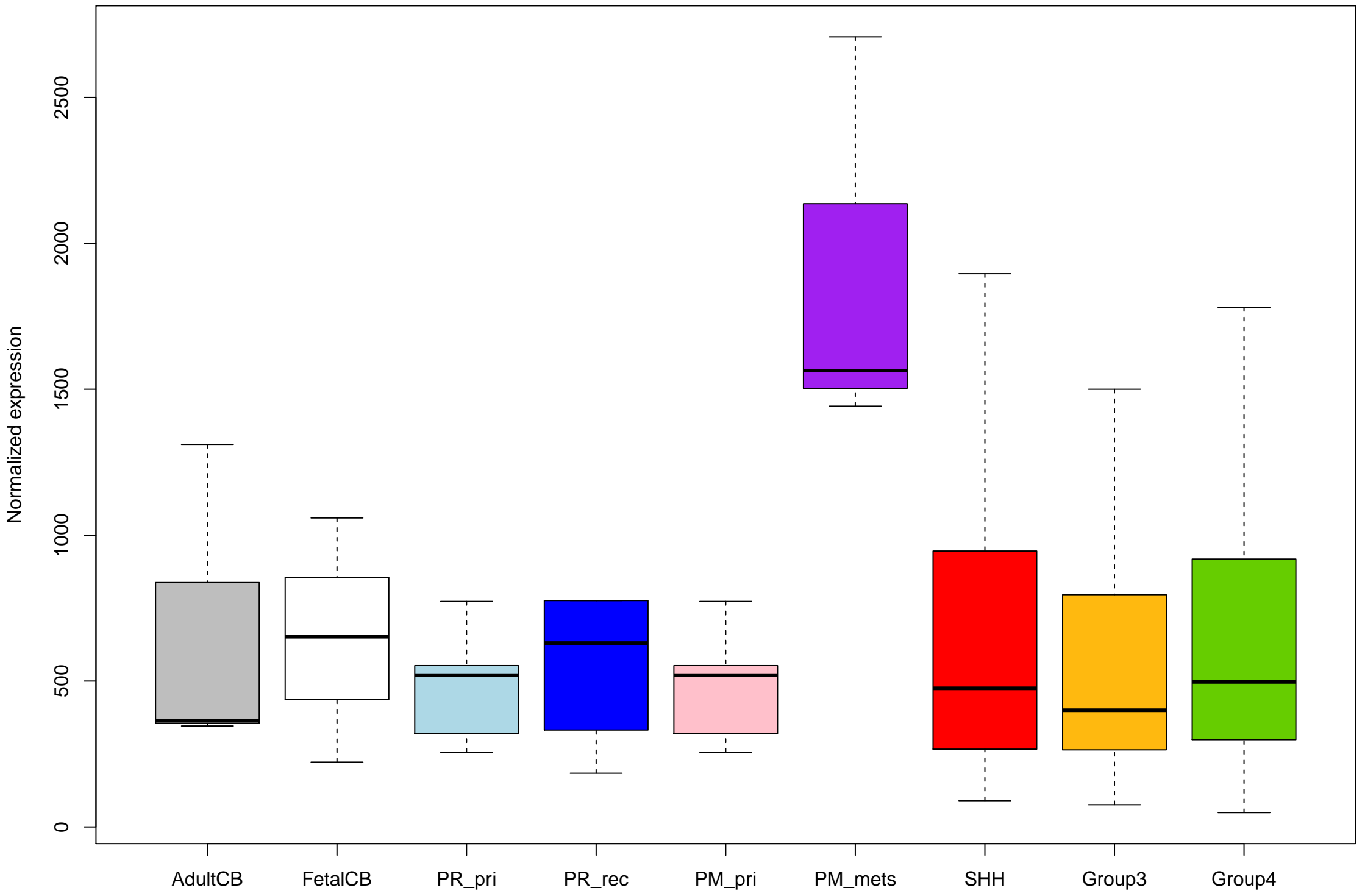
ENSG00000184005_ST6GALNAC3_+ expression (no outliers)
