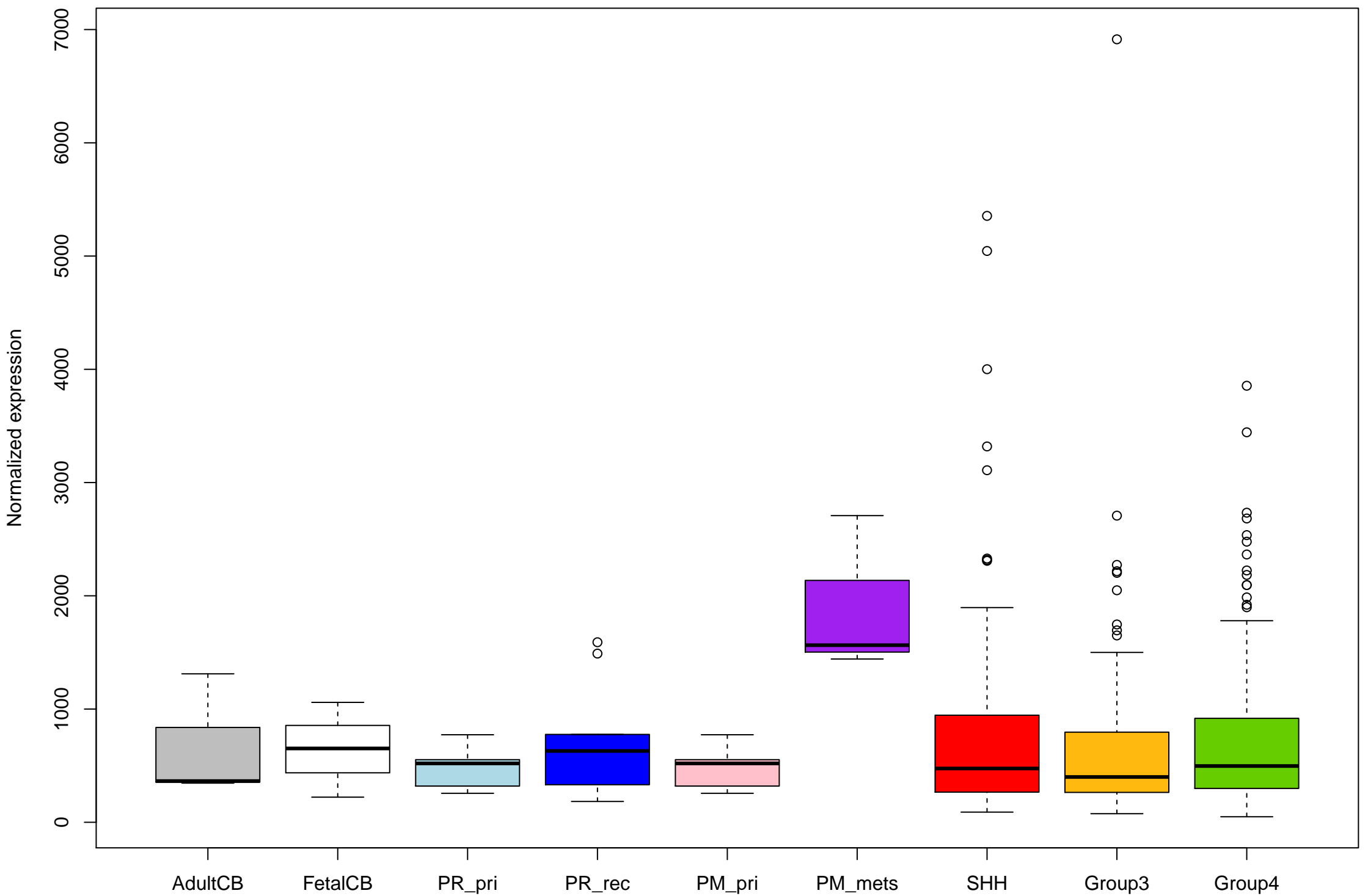
ENSG00000184005_ST6GALNAC3_+ expression (with outliers)
