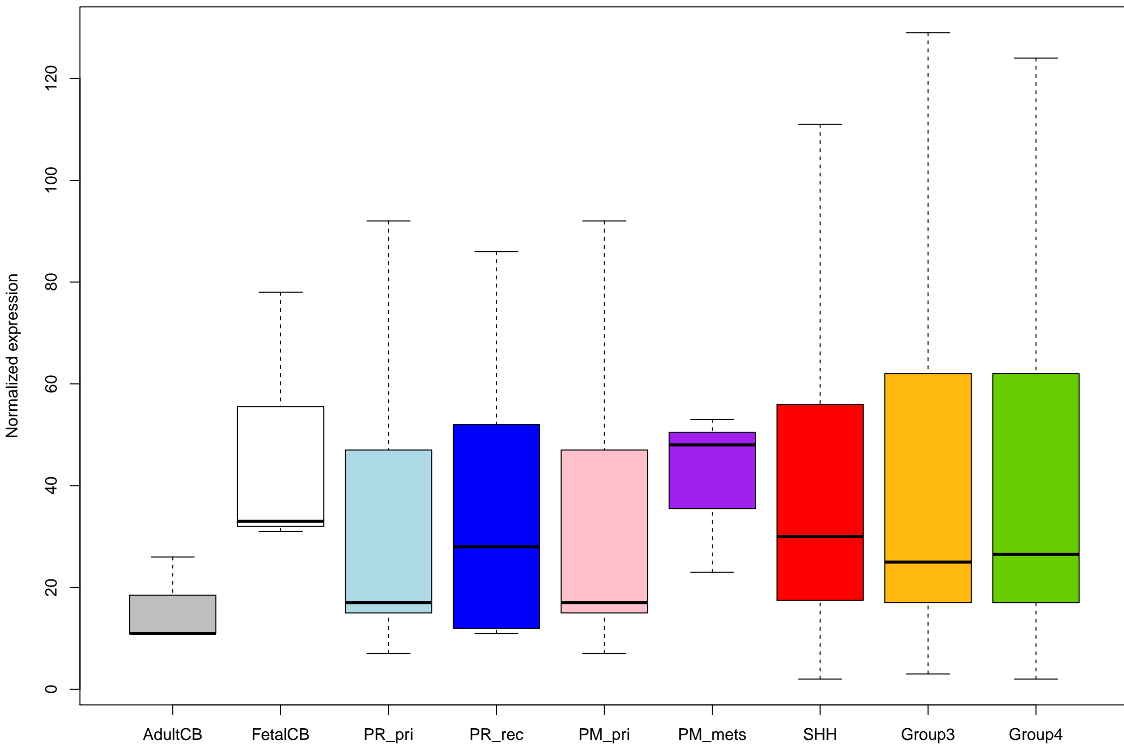
ENSG00000172058_SERF1A_+ expression (no outliers)
