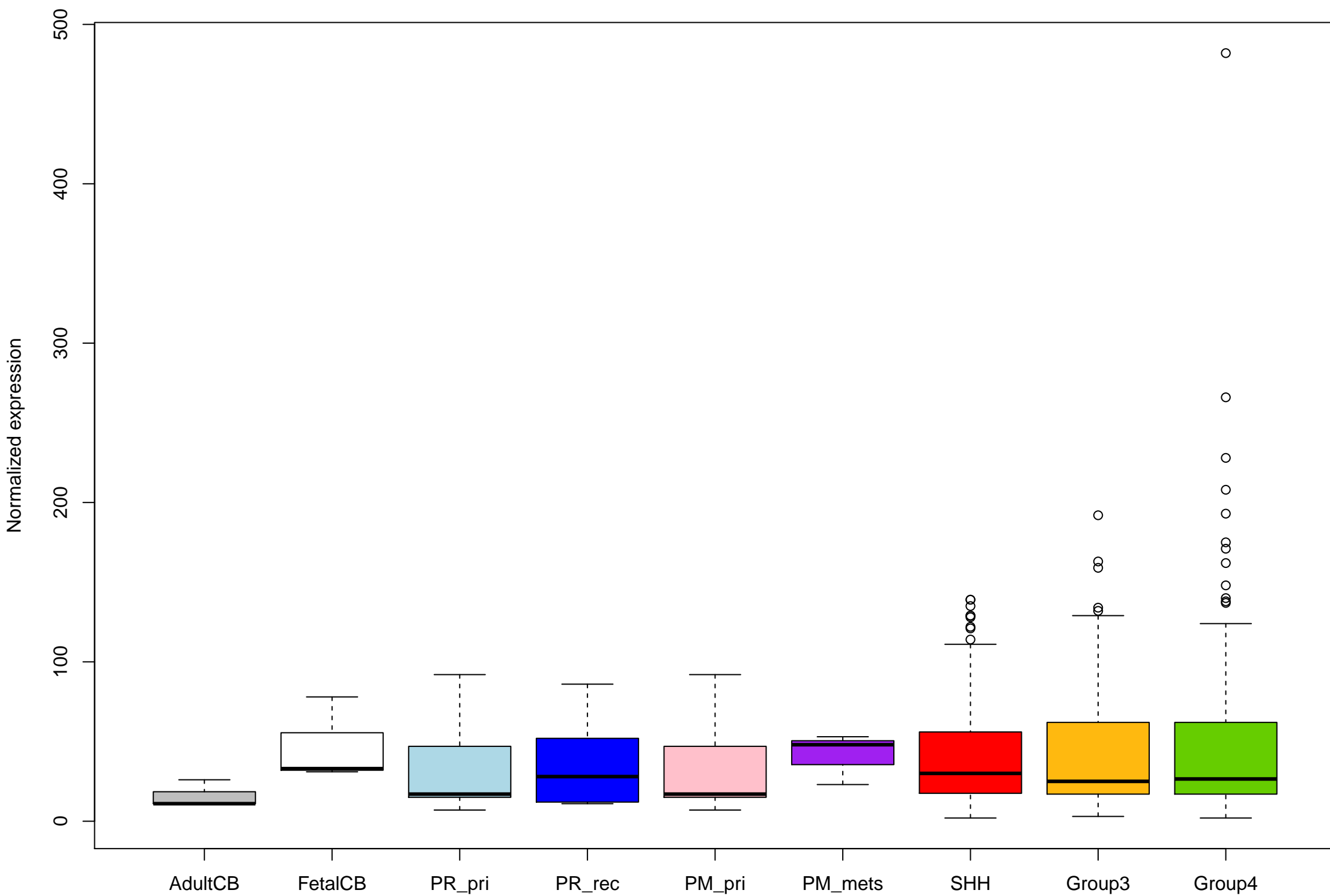
ENSG00000172058_SERF1A_+ expression (with outliers)
