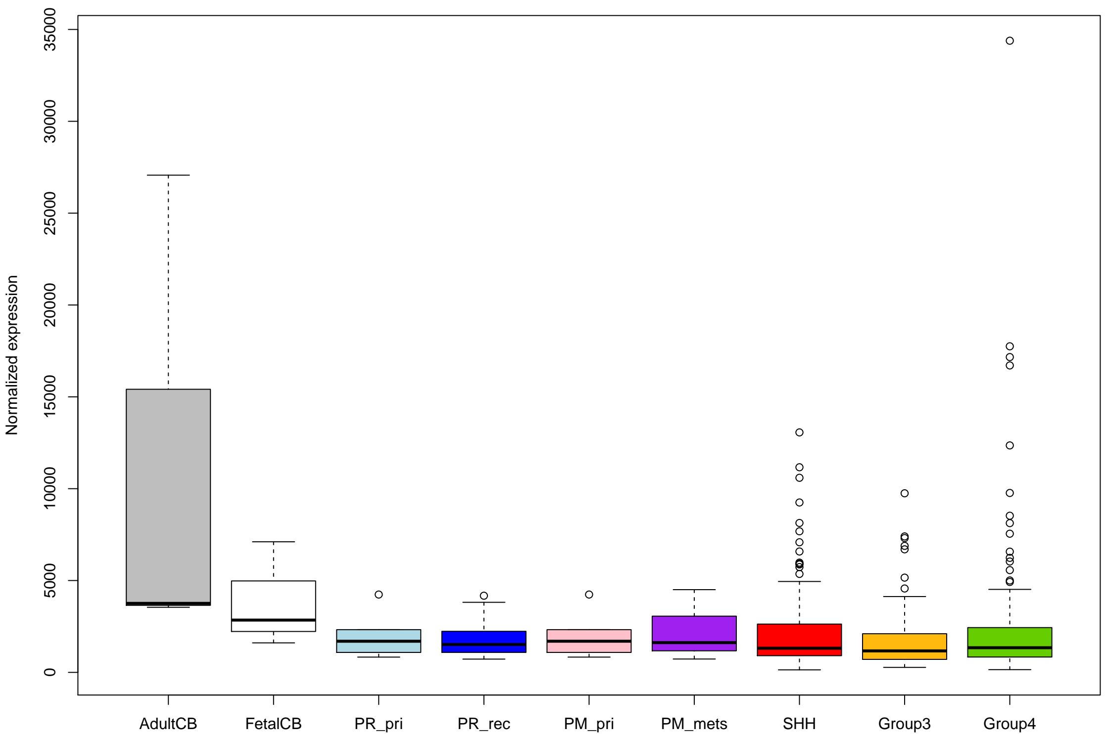
ENSG00000123096_SSPN_+ expression (with outliers)
