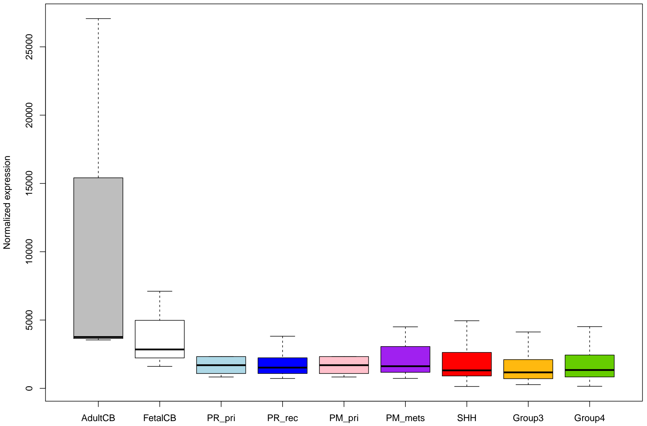
ENSG00000123096_SSPN_+ expression (no outliers)
